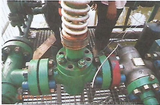
Fig.1: Damaged valve
